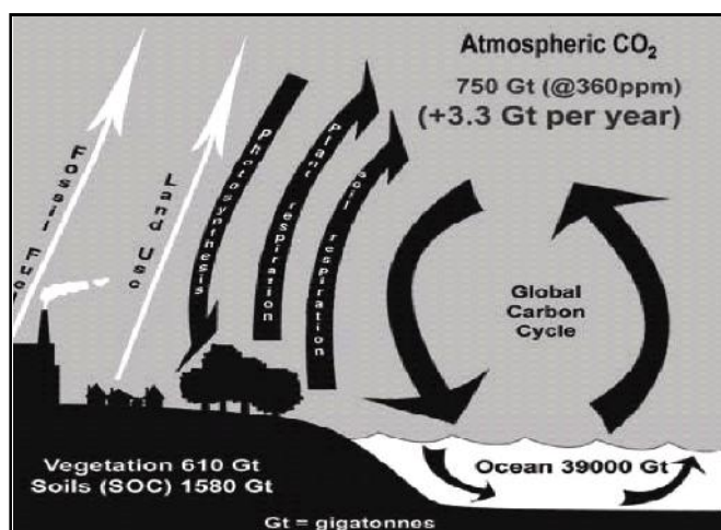
Fig. 1 : Soil organic carbon forms part of the natural carbon cycle (see Table 1). (White arrows indicate additional human outputs)
