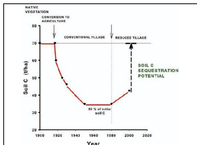
Fig. 2 : Historical change in SOC as a result of agricultural development, showing soil carbon sequestration potential
